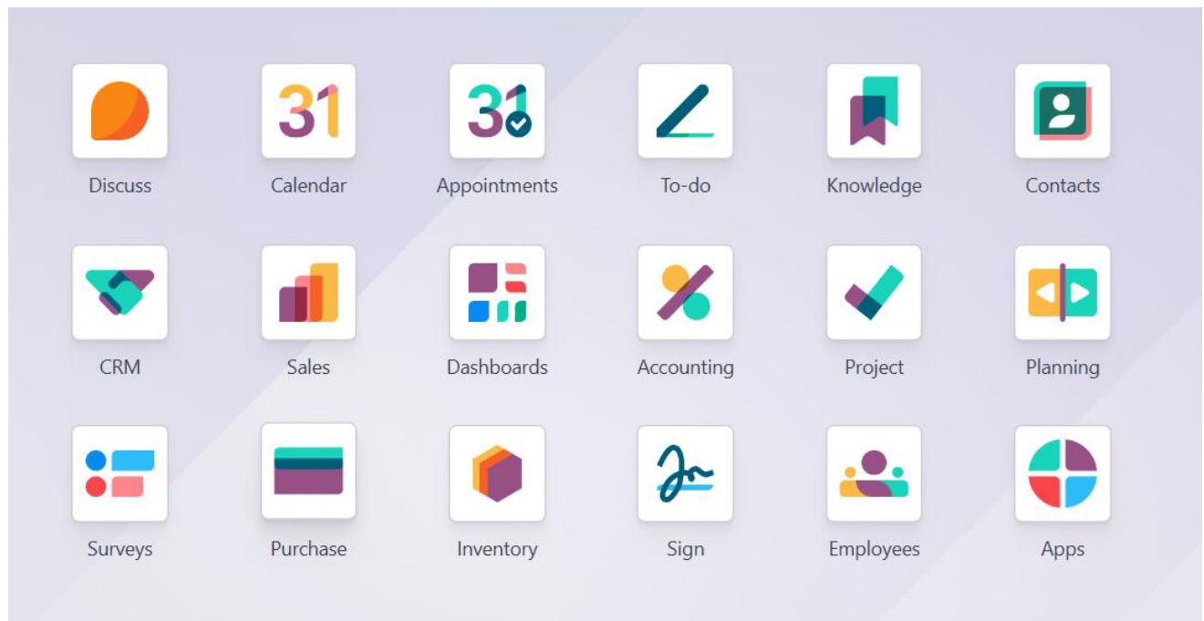
Figure 11. Image 3.2.3.1: Dashboard
