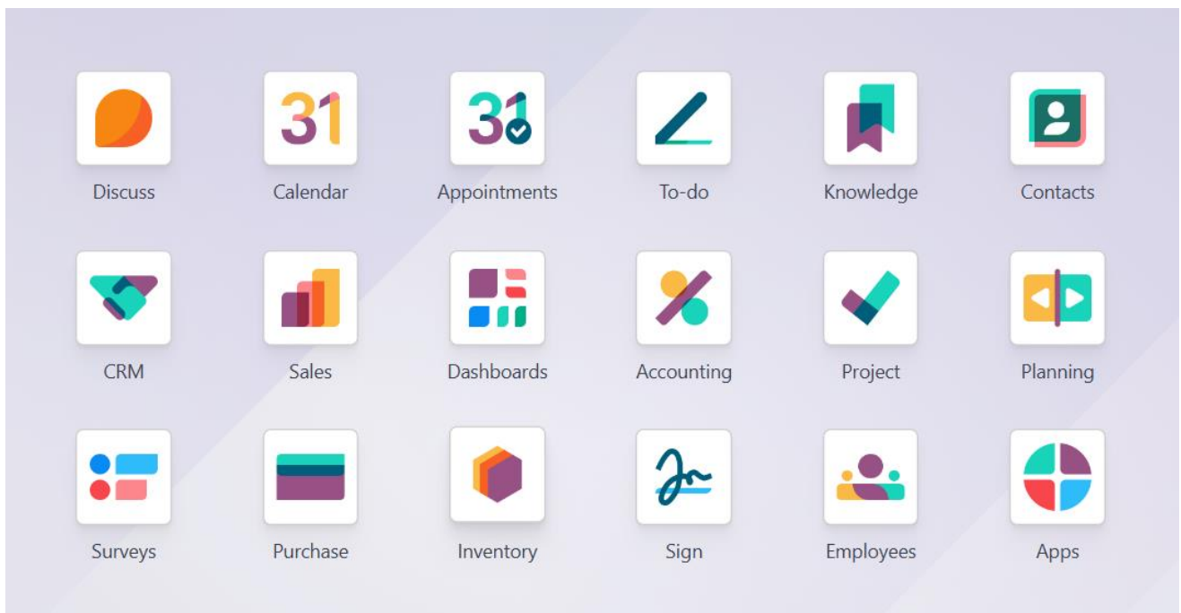
Figure 54: Image 3.5.3.1: Dashboard
