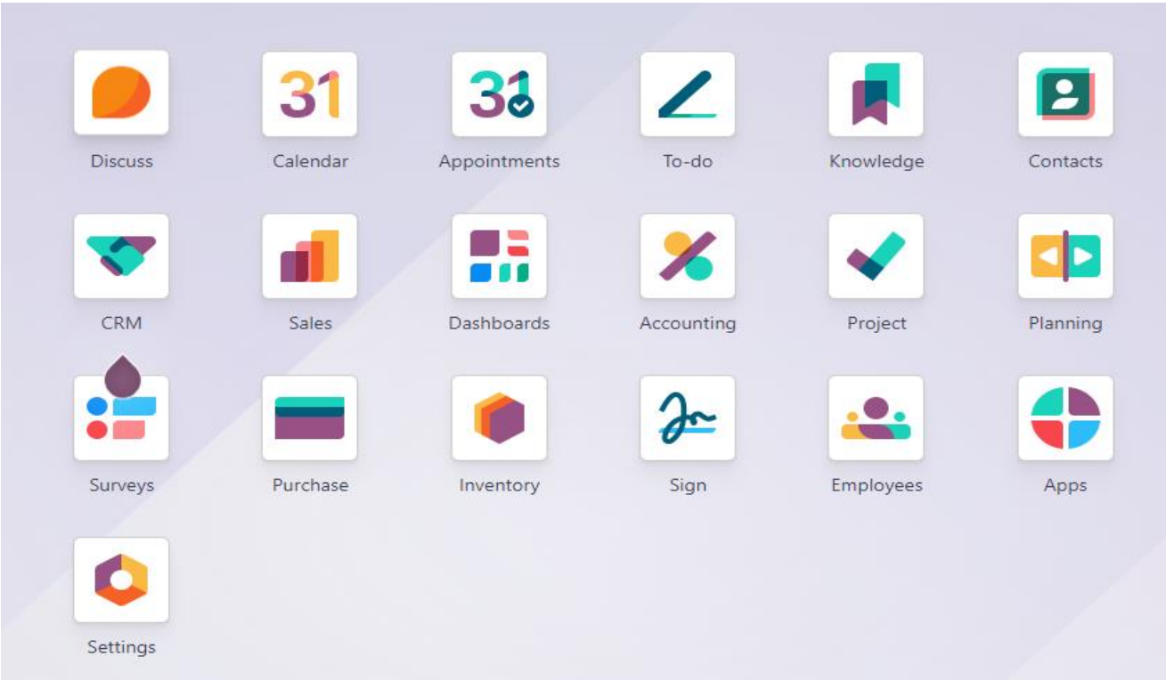
Figure 45: Image 3.4.3.5: Dashboard
