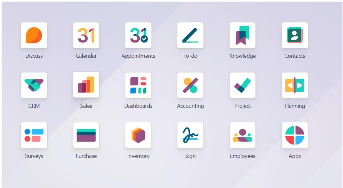
Figure 33. Image3.3.3.1: Dashboard
