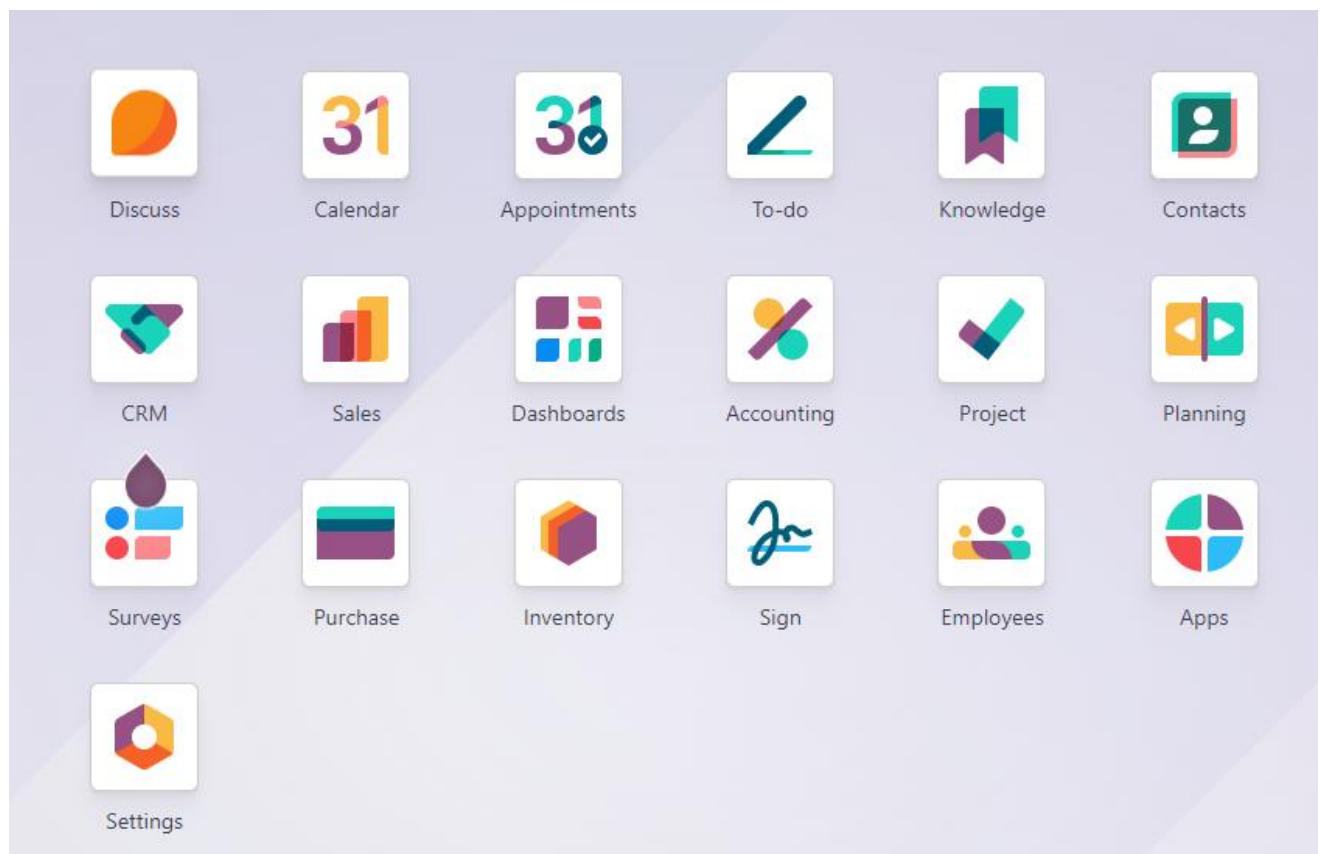
Figure 41: Image 3.4.3.1: Dashboard
